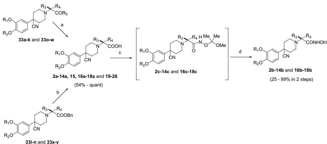
Scheme 3. Synthesis of 2a-14a , 15 , 16a-18a , 19-26 , 2b-14b , and 16b-18b . Reagents and conditions: (a) 2 N NaOHaq, EtOH; (b) \text{H}_2 , 10% Pd/C, MeOH; (c) EDC, HOBT, DMF, \text{NH}_2\text{OC}(\text{CH}_3)_2(\text{OCH}_3) ; (d) 2 N HClaq, MeOH.
