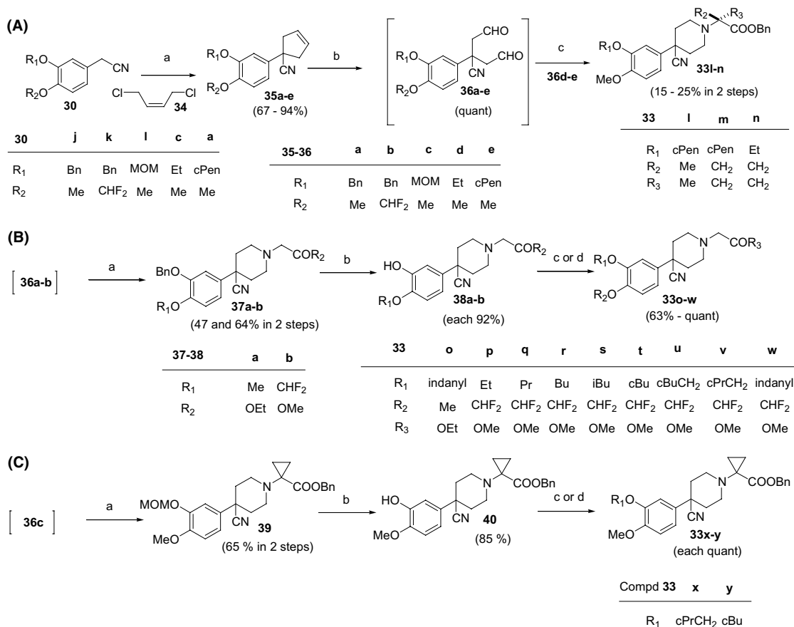
Scheme 2. (A) Synthesis of 33l-n . Reagents and conditions: (a) 34 , LiHMDS, THF, -78^{\circ}\text{C} ; (b) \text{O}_3 , \text{CH}_2\text{Cl}_2 , then \text{PPh}_3 , -78^{\circ}\text{C} ; (c) \text{NaBH}(\text{OAc})_3 , AcOH, DCE, or DMF, \text{NH}_2\text{CR}_2\text{R}_3\text{COOBn} . (B) Synthesis of 33o-w . Reagents and conditions: (a) \text{NaBH}(\text{OAc})_3 , AcOH, DCE, or DMF, \text{NH}_2\text{CH}_2\text{COR}_5 ; (b) \text{H}_2 , 10% Pd/C, MeOH; (c) alcohol, DEAD, \text{PPh}_3 , THF; (d) alkyl halide, \text{K}_2\text{CO}_3 , DMF. (C) Synthesis of 33x-y . Reagents and conditions: (a) \text{NaBH}(\text{OAc})_3 , AcOH, DCE, or DMF, \text{NH}_2\text{C}(\text{CH}_2)_2\text{COOBn} ; (b) 4 N HCl/EtOAc, \text{CH}_2\text{Cl}_2 ; (c) alcohol, DEAD, \text{PPh}_3 , THF; (d) alkyl halide, \text{K}_2\text{CO}_3 , DMF.
