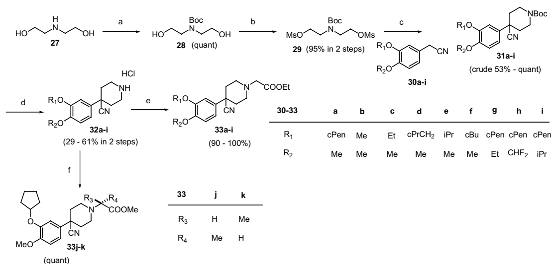
Scheme 1. Synthesis of 33a–k . Reagents and conditions: (a) Boc 2 O, CH 2 Cl 2 , 0°C; (b) MsCl, Et 3 N, CH 2 Cl 2 , –78°C; (c) 30a–i , LiHMDS, THF, –78°C; (d) TFA, C 6 H 5 SCl 3 , CH 2 Cl 2 , then 4N HCl/EtOAc; (e) K 2 CO 3 , BrCH 2 COOEt, DMF; (f) methyl- S -(-)-lactate or methyl- R -(+)-lactate, Tf 2 O, CH 2 Cl 2 , 2,6-lutidine, Et 3 N.
