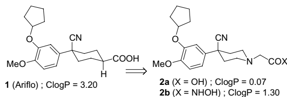
Figure 1. Molecular design of hydrophilic molecules.
